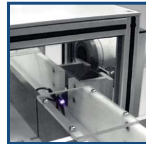
Detailed view of corona treating process
